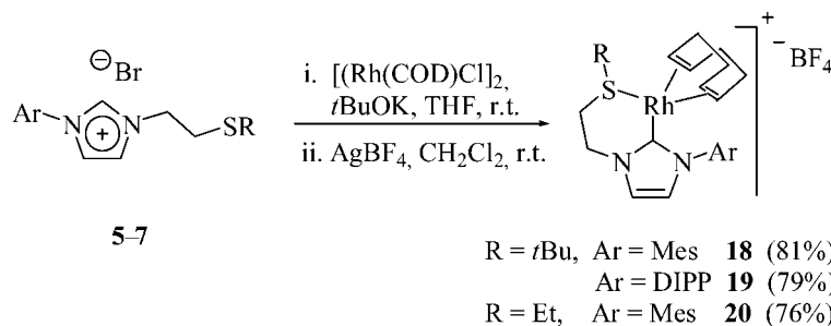
Scheme 4. Synthesis of rhodium(I) complexes.
