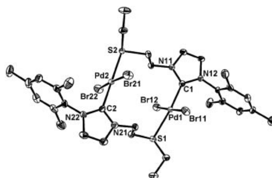
Figure 4. An ORTEP view of compound 17 . Ellipsoids are represented at the 30% probability level. Hydrogen atoms and a co-crystallised THF molecule are omitted for clarity. Selected bond lengths [Å] and angles [°]: Pd1–C1 1.990(4), Pd2–C2 1.983(4), Pd1–S1 2.3731(9), Pd2–S2 2.3622(9), Br21–Pd2–Br22 175.50(2), C1–Pd1–S1 173.10(12).
